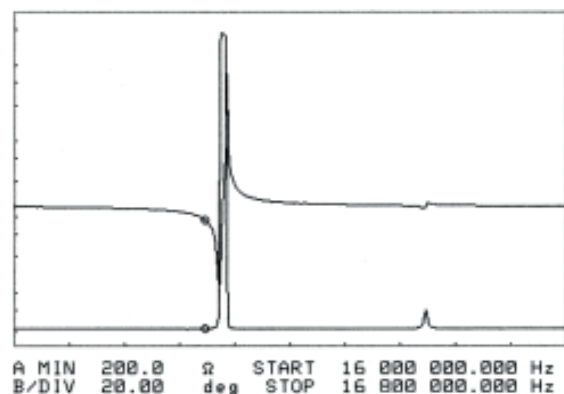
Figure 4: Impedance as a function of frequency for a (roughly) 16MHz CX-4 (obtained using a HP 4194A). Note the lack of any significant and harmonic modes in this particular design.
