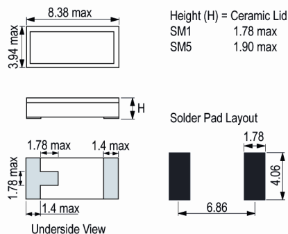
Outline (mm) -C-SM1 = Gold Plated (RoHS)
