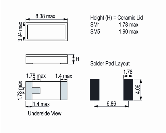
Outline (mm) -C-SM1 = Gold Plated (RoHS)
