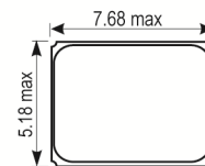
Outline (mm) A-SM1 = 5000G, Gold Plated (RoHS)
