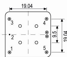
Underside View
