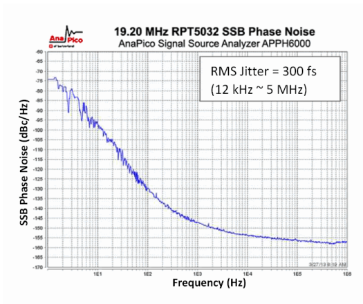
Example Phase Noise @ 19.20MHz
