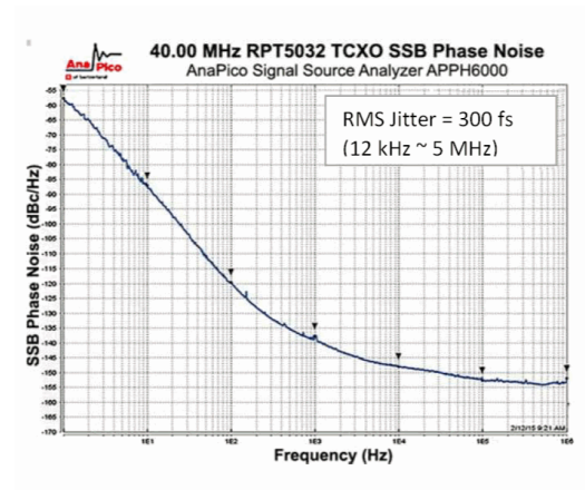
Example Phase Noise @ 40.00MHz
